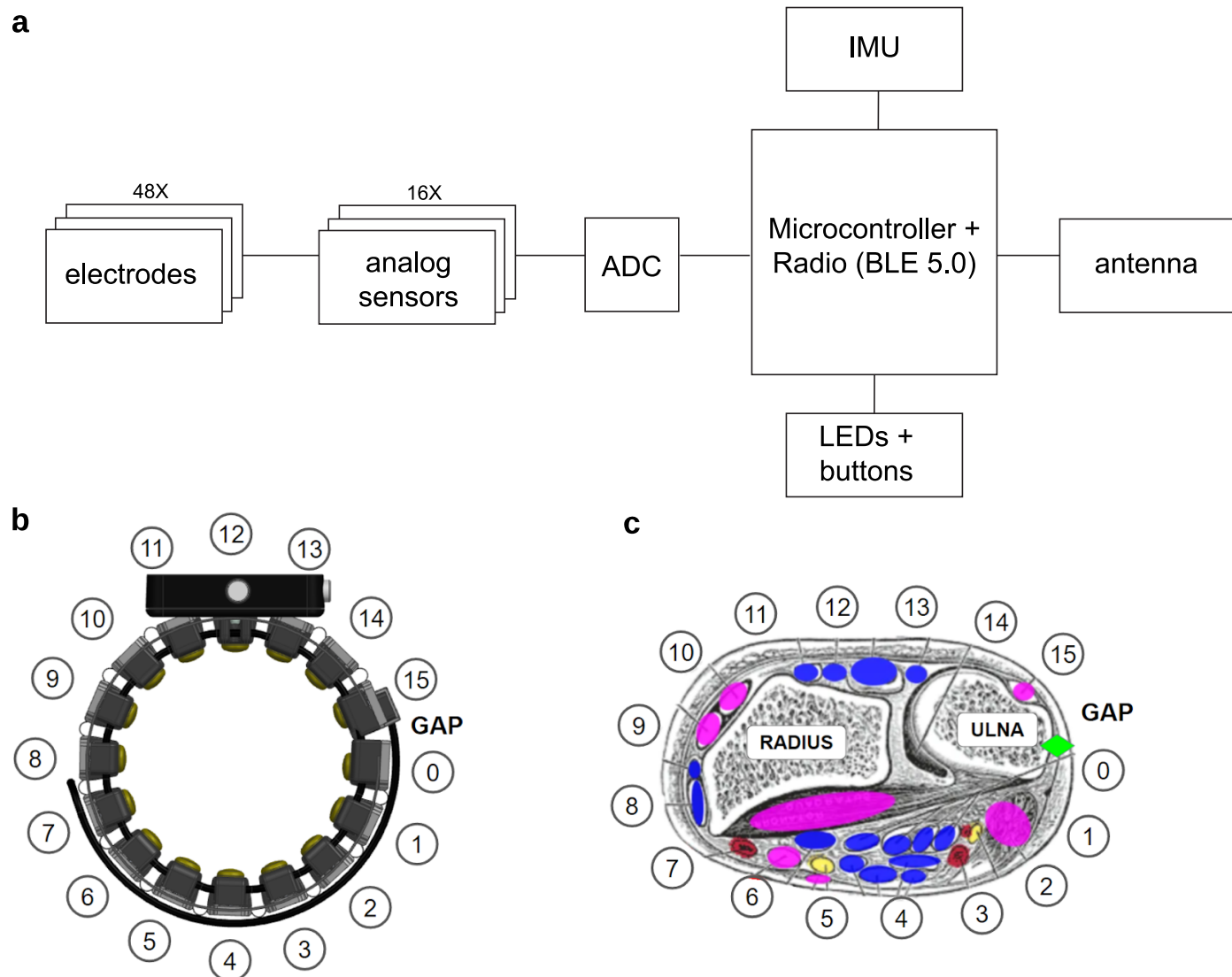
Extended Data Fig. 1 | Schematic and anatomical interfacing of sEMG Research Device. a , The sEMG Research Device electrical system architecture. The sEMG-RD uses 48 pogo-pin style round electrodes in order to provide good comfort and contact quality. The 48 channels are configured into 16 bipolar channels arranged proximo-distally, with the remainder electrodes serving as either shield or ground. Each electrode is 6.5 mm in diameter (gold plated brass). For each differential sensing channel (16 in total), centre-to-centre spacing between paired sensing electrodes is 20 mm. The sEMG-RD has low noise analog sensors with input-referred RMS noise of 2.46 \mu\text{V}_{\text{rms}} , measured during benchtop testing with differential inputs shorted to their mid-point voltage. With analog sensors' nominal gain value of 190 and Analog to Digital Converter's (ADC) full-scale range of 2.5 V, the sEMG-RD offers a dynamic range of approximately 65.5 dB. Each channel is sampled at 2000 Hz. The Inertial Measurement Unit (IMU) functional block includes sensors of 3-axis accelerometer, 3-axis gyroscope, and 3-axis magnetometer sampled at 100 Hz. We note that the IMU was not utilized for any online or offline experiments described in this manuscript. The microcontroller facilitates the transfer of unprocessed data from all ADCs and IMU directly to the bluetooth radio. No skin preparation or gels are needed for using the sEMG-RD, because its analog
